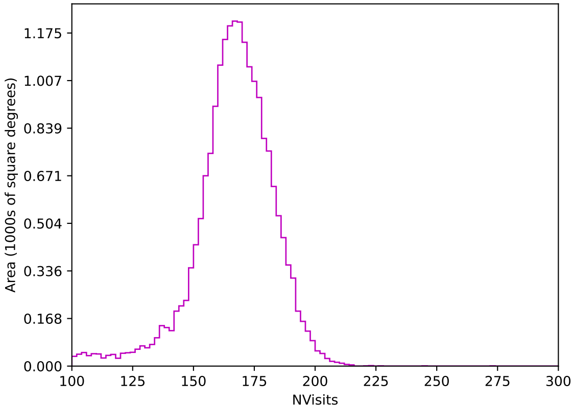
start_date_do90v3.4_10yrs All sky z band: NVisits
