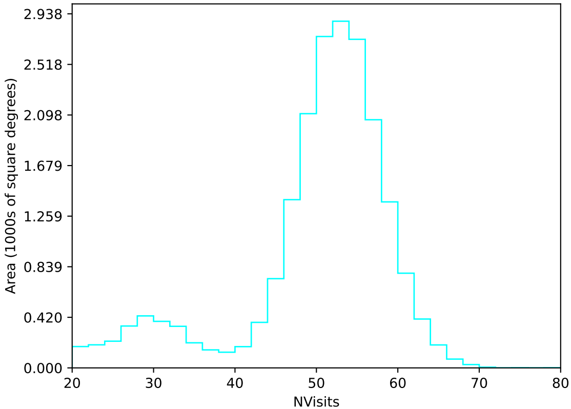
start_date_do90v3.4_10yrs All sky u band: NVisits
