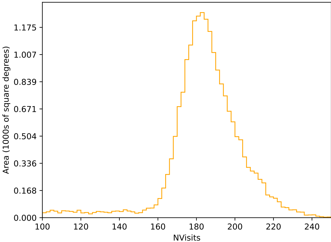
start_date_do90v3.4_10yrs All sky r band: NVisits
