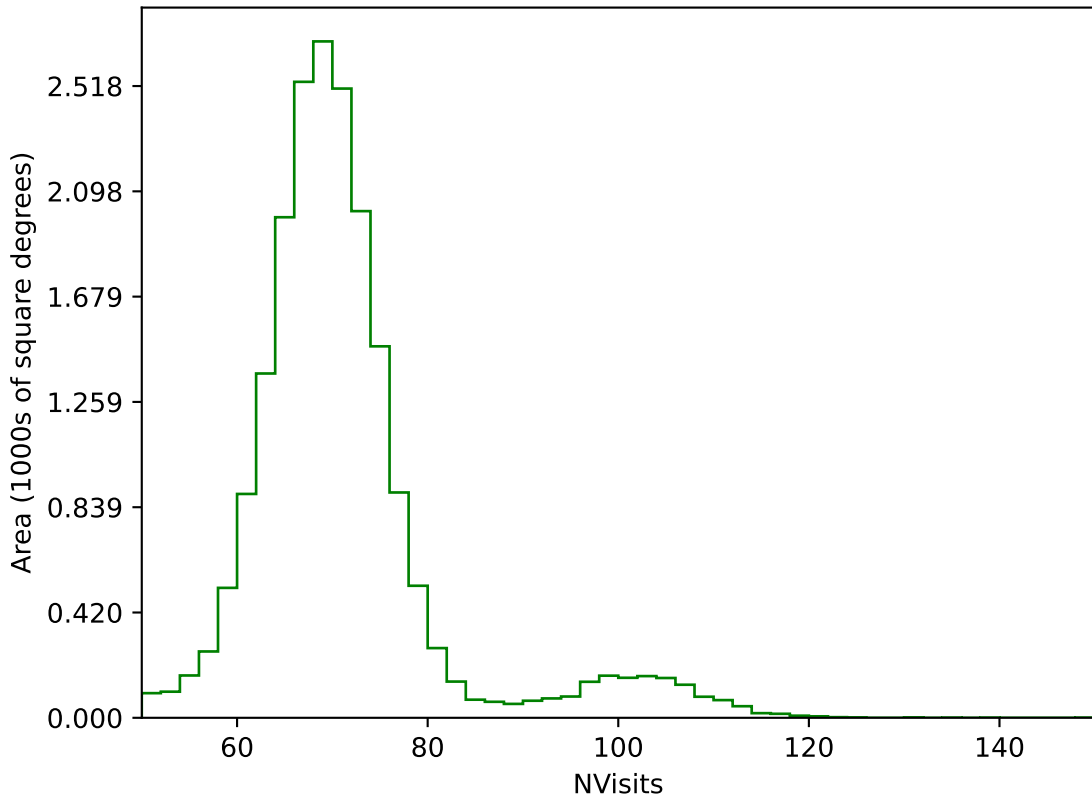
start_date_do90v3.4_10yrs All sky g band: NVisits
