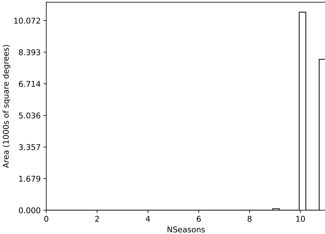
start_date_do90v3.4_10yrs WFD all bands: NSeasons
