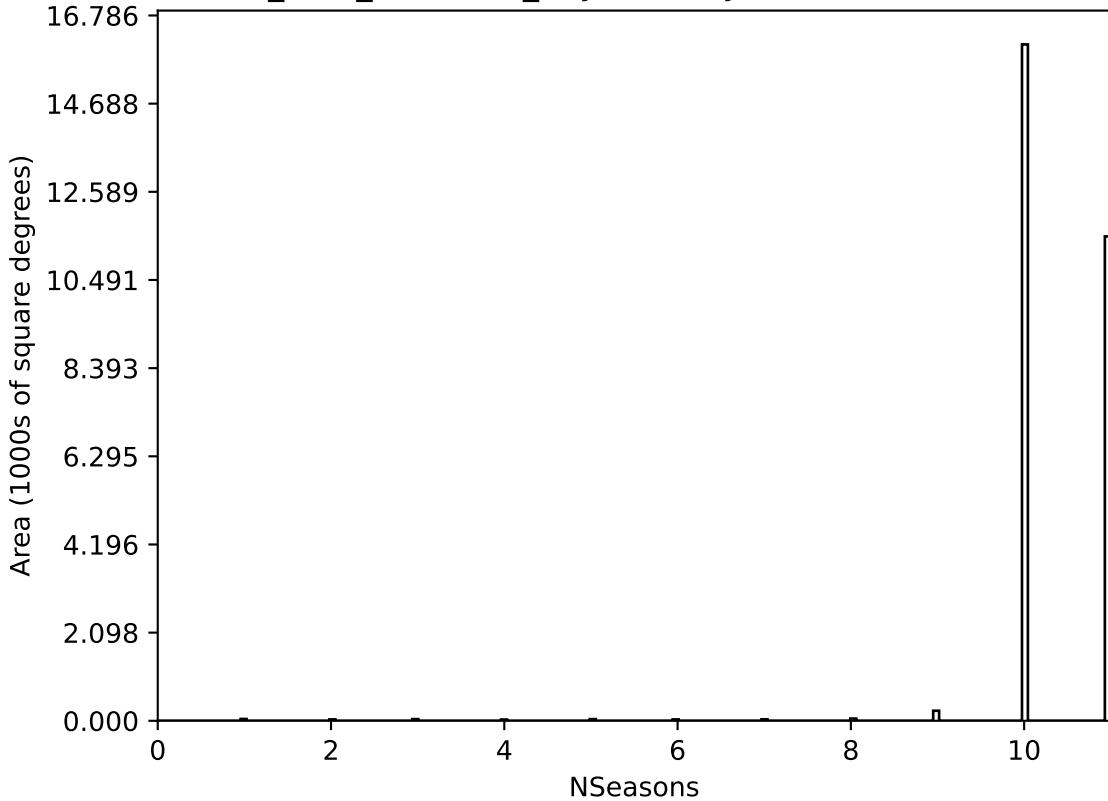
start_date_do90v3.4_10yrs All sky all bands: NSeasons
