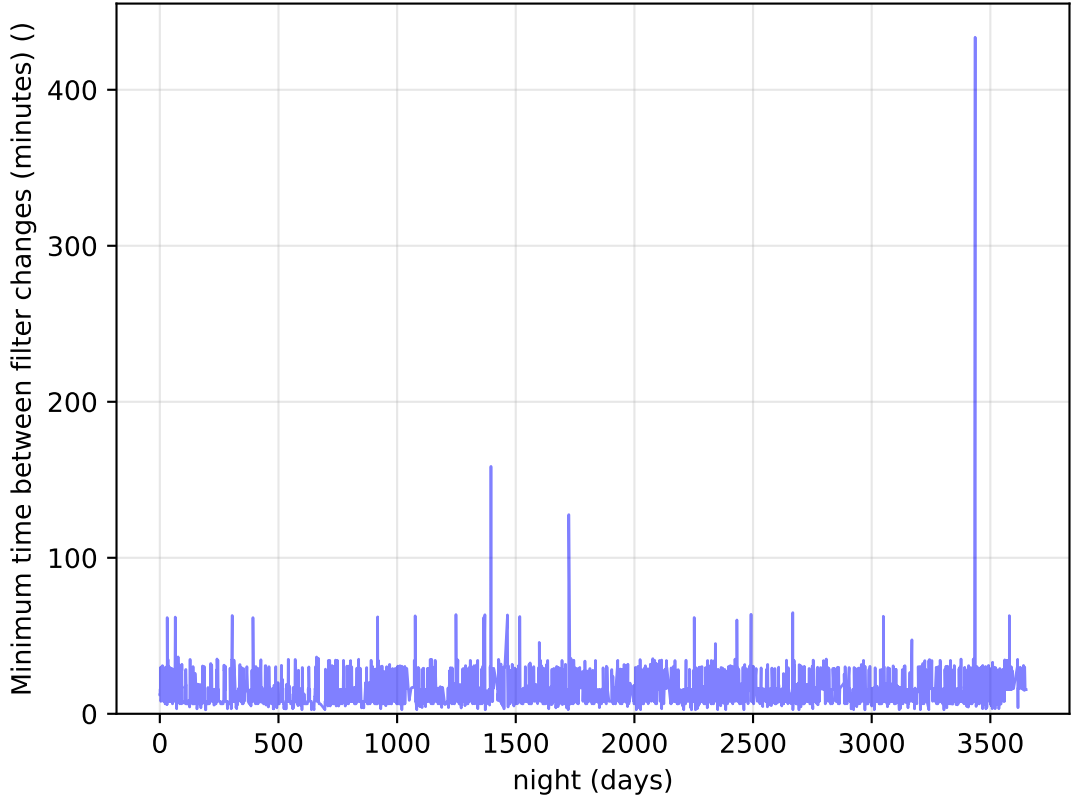
start_date_do90v3.4_10yrs Per Night: Minimum time between filter changes (minutes)
