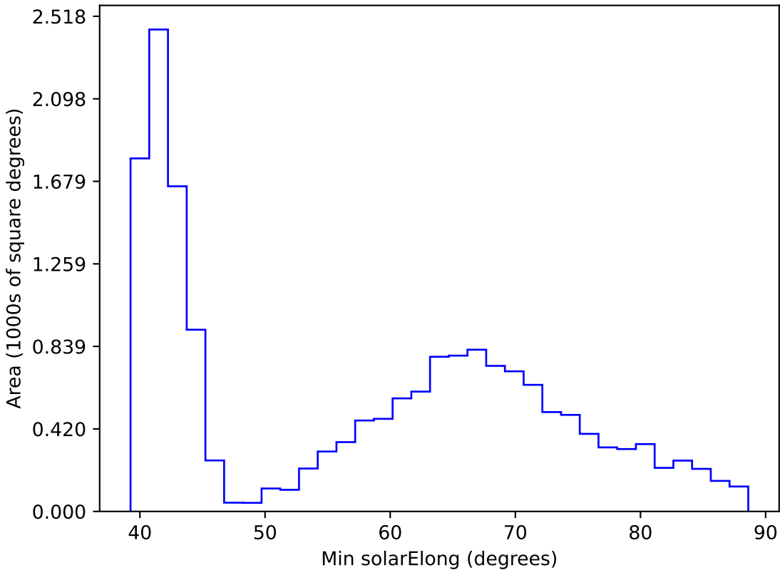
start_date_do90v3.4_10yrs WFD r band: Min solarElong
