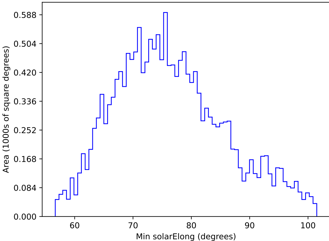
start_date_do90v3.4_10yrs WFD g band: Min solarElong
