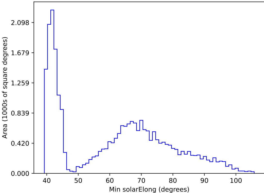
start_date_do90v3.4_10yrs All sky r band: Min solarElong
