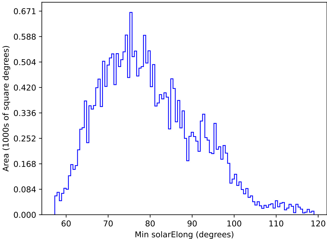
start_date_do90v3.4_10yrs All sky g band: Min solarElong
