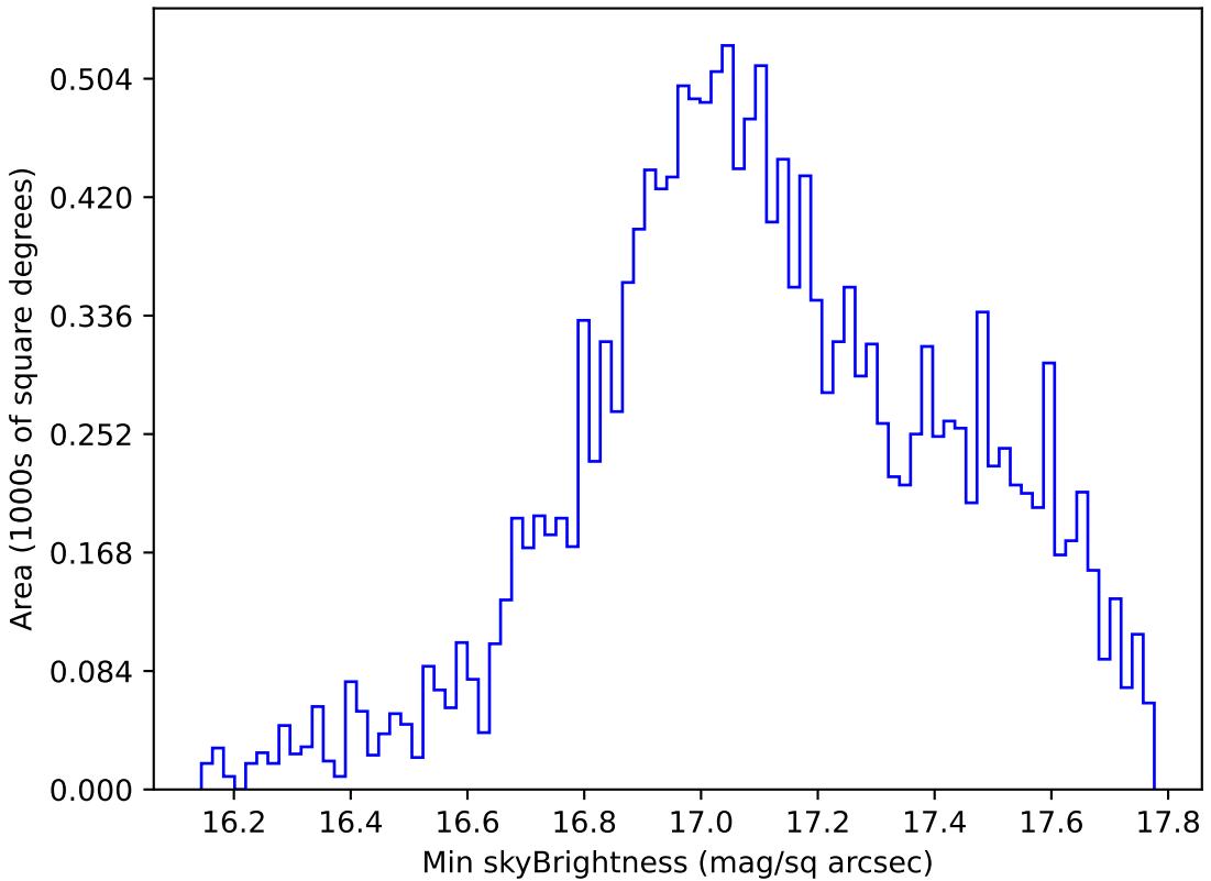
start_date_do90v3.4_10yrs WFD y band: Min skyBrightness
