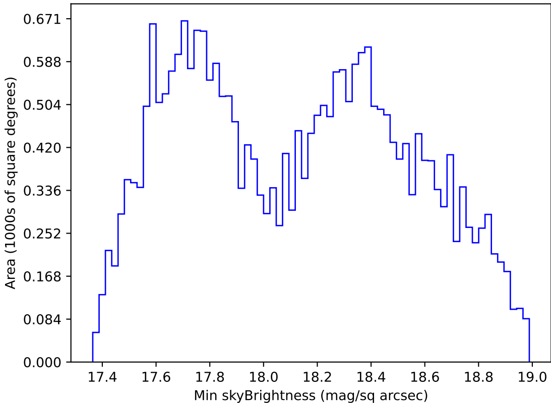
start_date_do90v3.4_10yrs All sky i band: Min skyBrightness
