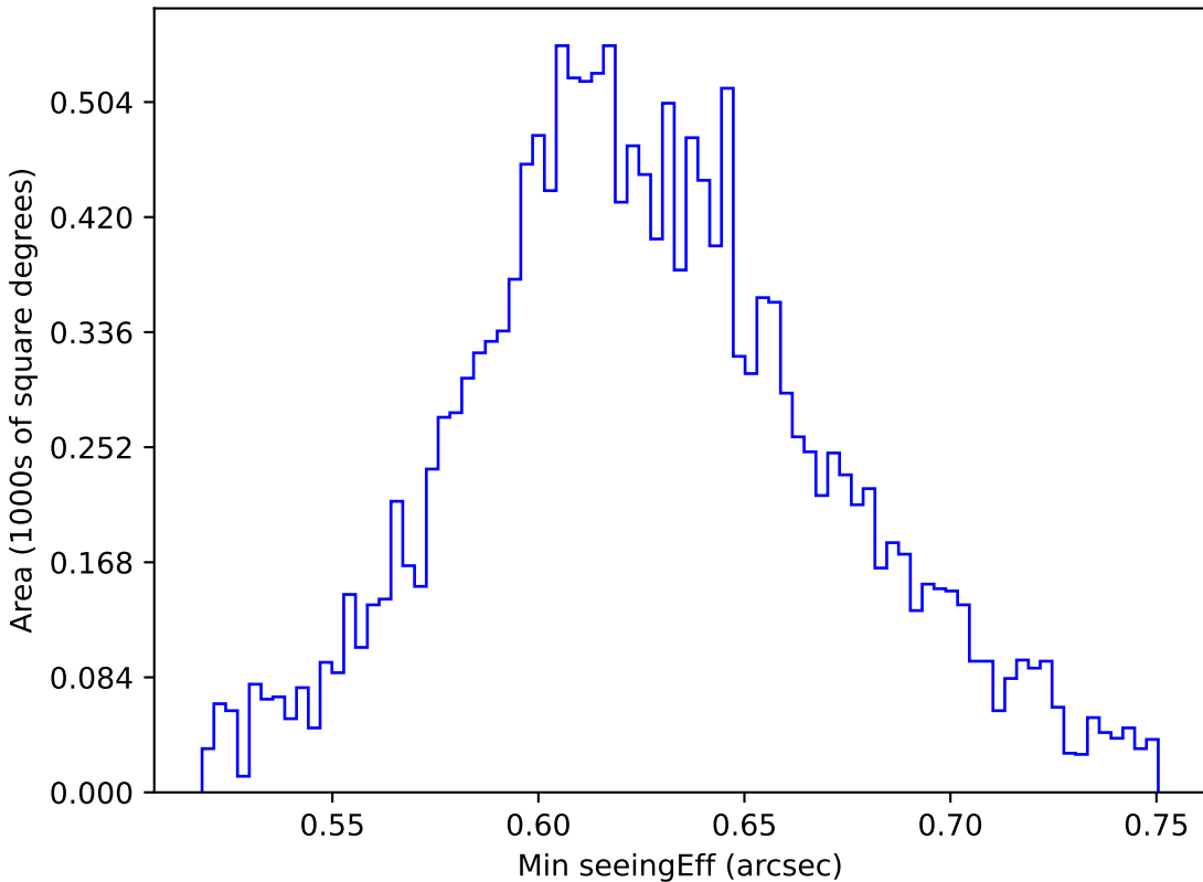
start_date_do90v3.4_10yrs WFD y band: Min seeingEff
