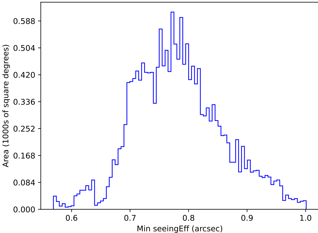
start_date_do90v3.4_10yrs WFD u band: Min seeingEff
