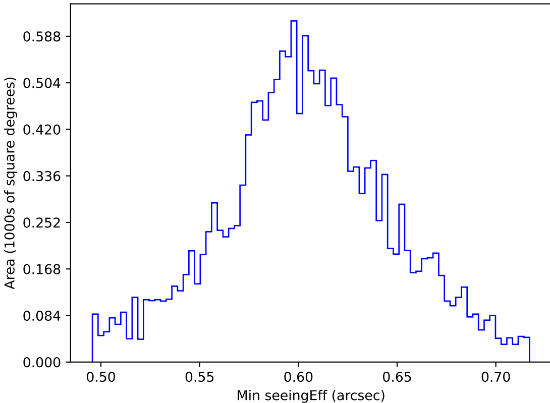
start_date_do90v3.4_10yrs WFD i band: Min seeingEff
