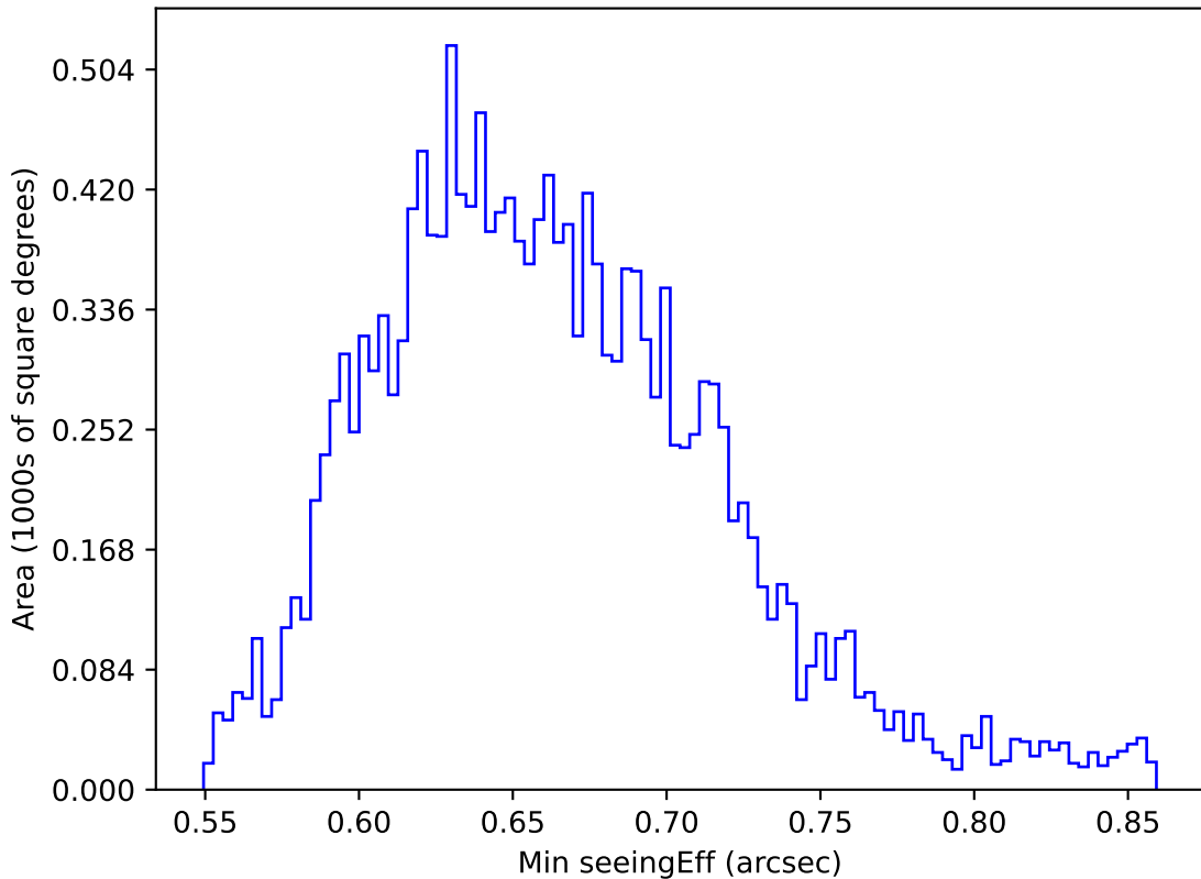
start_date_do90v3.4_10yrs WFD g band: Min seeingEff
