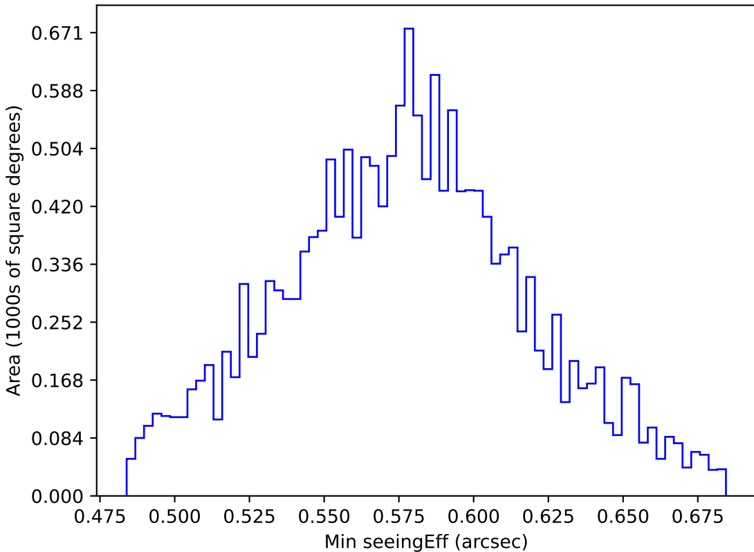
start_date_do90v3.4_10yrs WFD all bands: Min seeingEff
