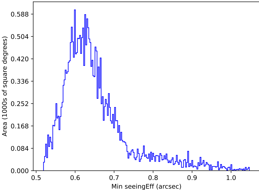
start_date_do90v3.4_10yrs All sky z band: Min seeingEff
