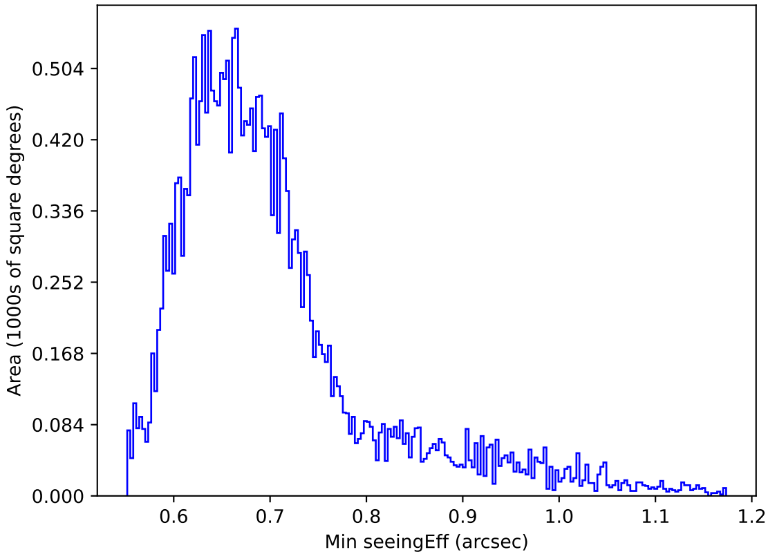
start_date_do90v3.4_10yrs All sky g band: Min seeingEff
