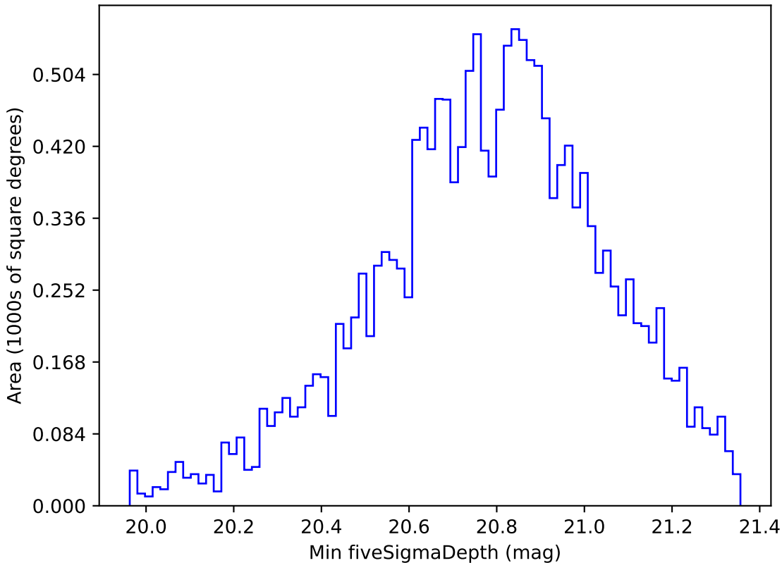
start_date_do90v3.4_10yrs WFD all bands: Min fiveSigmaDepth
