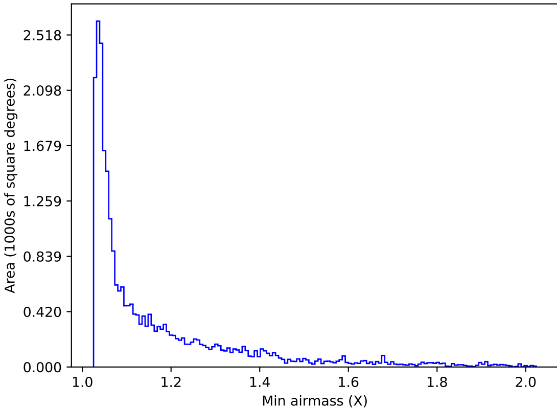
start_date_do90v3.4_10yrs Yr 1 z band: Min airmass
