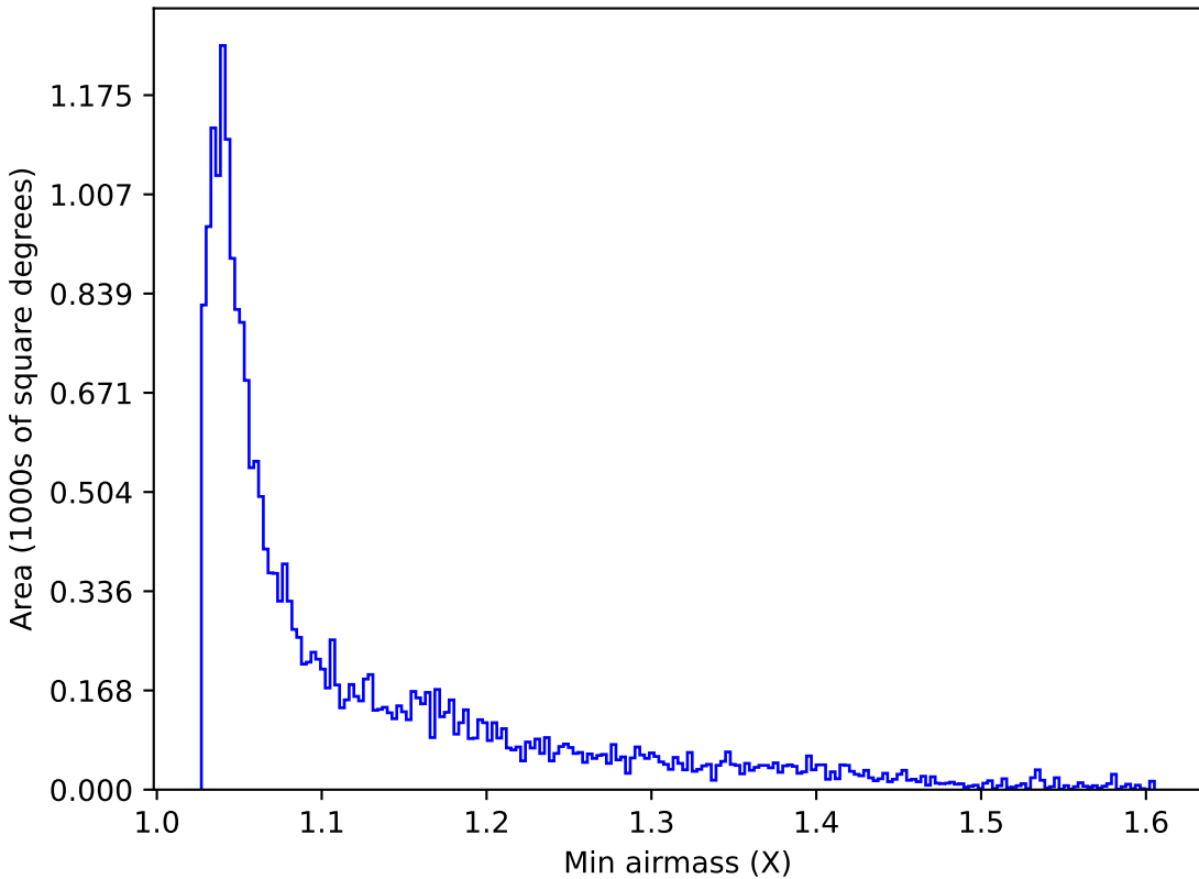
start_date_do90v3.4_10yrs Yr 1 y band: Min airmass
