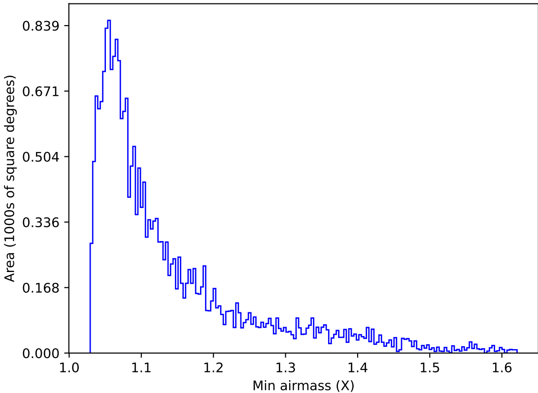
start_date_do90v3.4_10yrs Yr 1 u band: Min airmass
