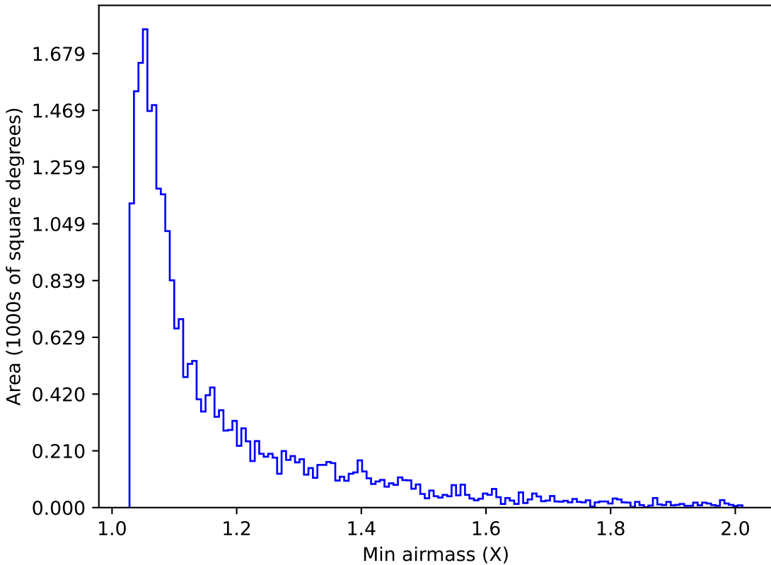
start_date_do90v3.4_10yrs Yr 1 g band: Min airmass
