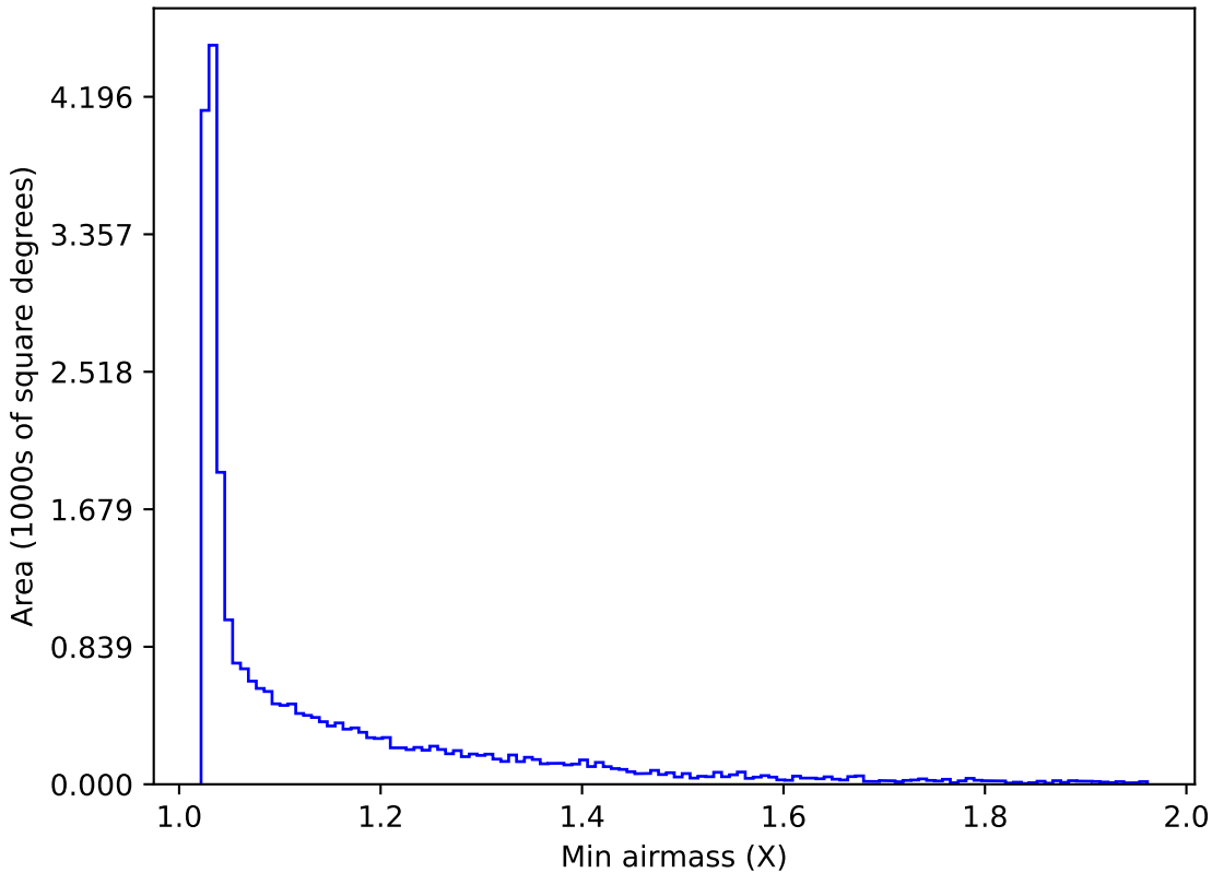
start_date_do90v3.4_10yrs Yr 1 all bands: Min airmass
