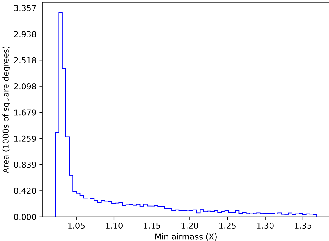
start_date_do90v3.4_10yrs WFD y band: Min airmass
