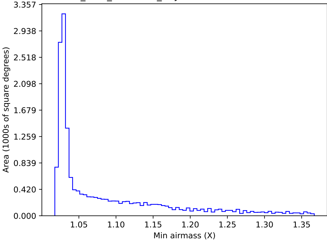
start_date_do90v3.4_10yrs WFD i band: Min airmass
