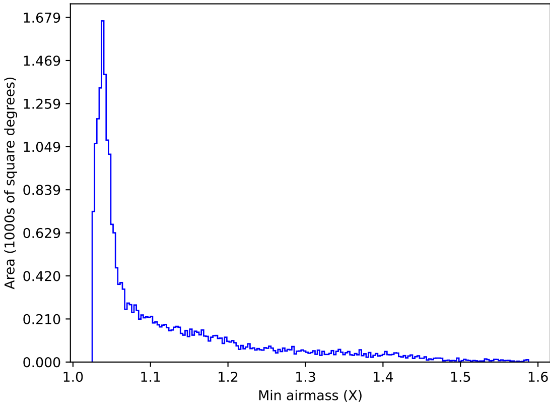
start_date_do90v3.4_10yrs All sky u band: Min airmass
