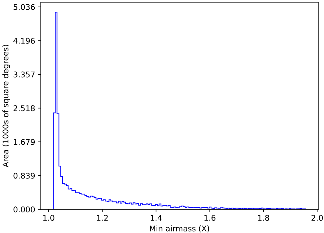
start_date_do90v3.4_10yrs All sky r band: Min airmass
