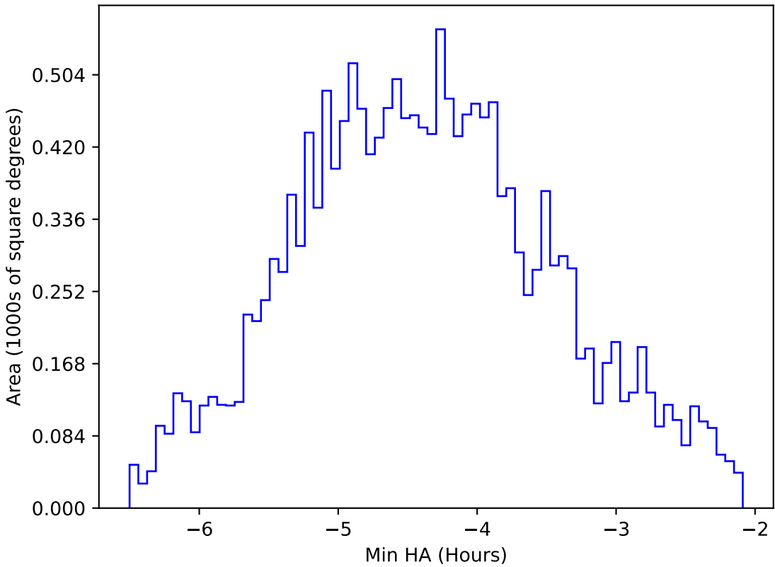
start_date_do90v3.4_10yrs WFD z band: Min HA
