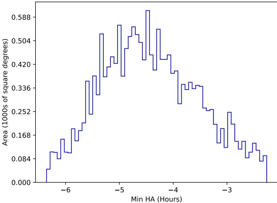
start_date_do90v3.4_10yrs WFD r band: Min HA
