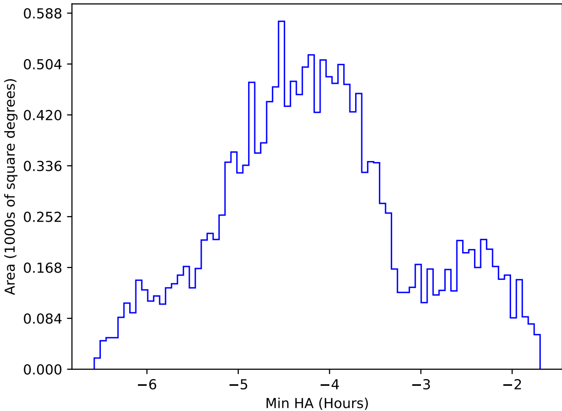
start_date_do90v3.4_10yrs WFD g band: Min HA
