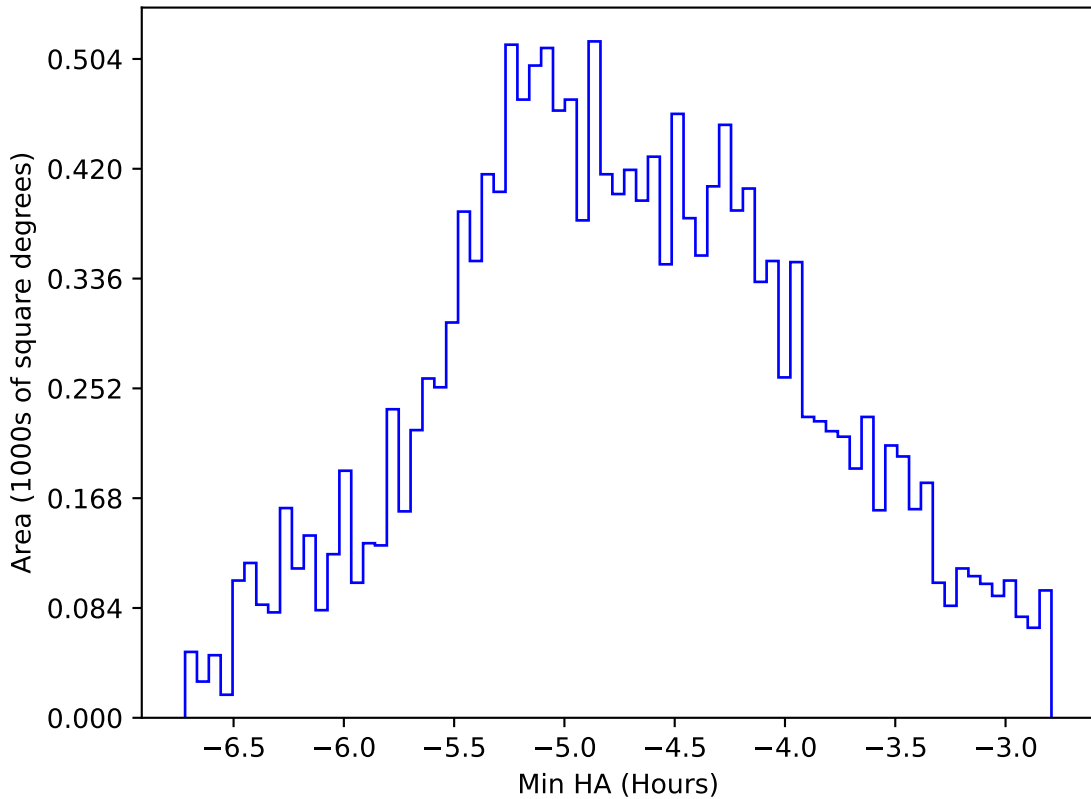
start_date_do90v3.4_10yrs WFD all bands: Min HA
