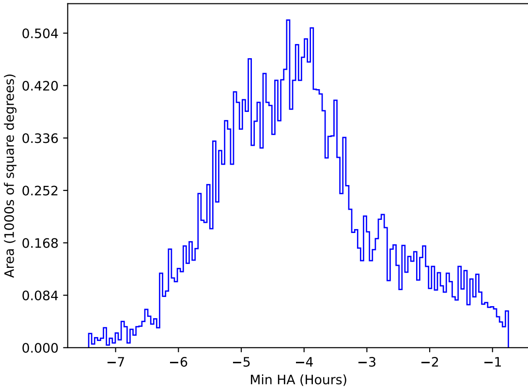
start_date_do90v3.4_10yrs All sky z band: Min HA
