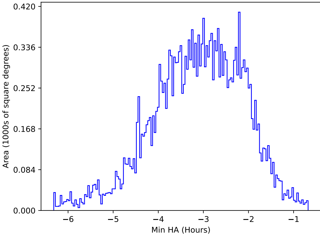
start_date_do90v3.4_10yrs All sky u band: Min HA
