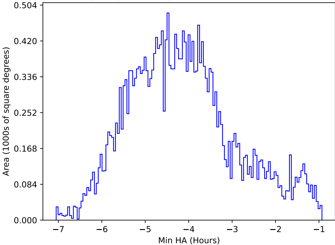
start_date_do90v3.4_10yrs All sky r band: Min HA
