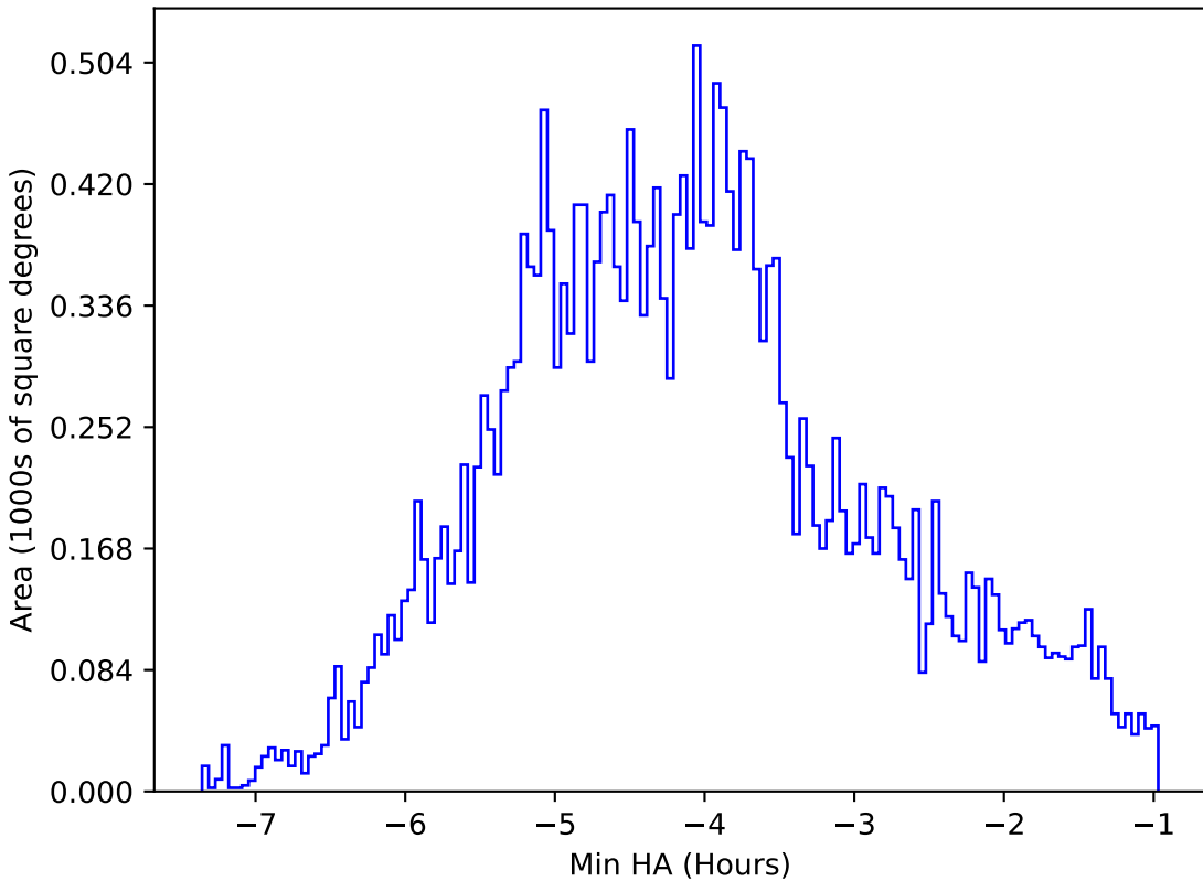
start_date_do90v3.4_10yrs All sky i band: Min HA
