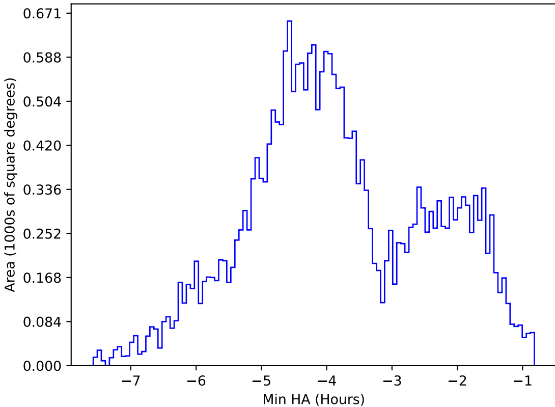
start_date_do90v3.4_10yrs All sky g band: Min HA
