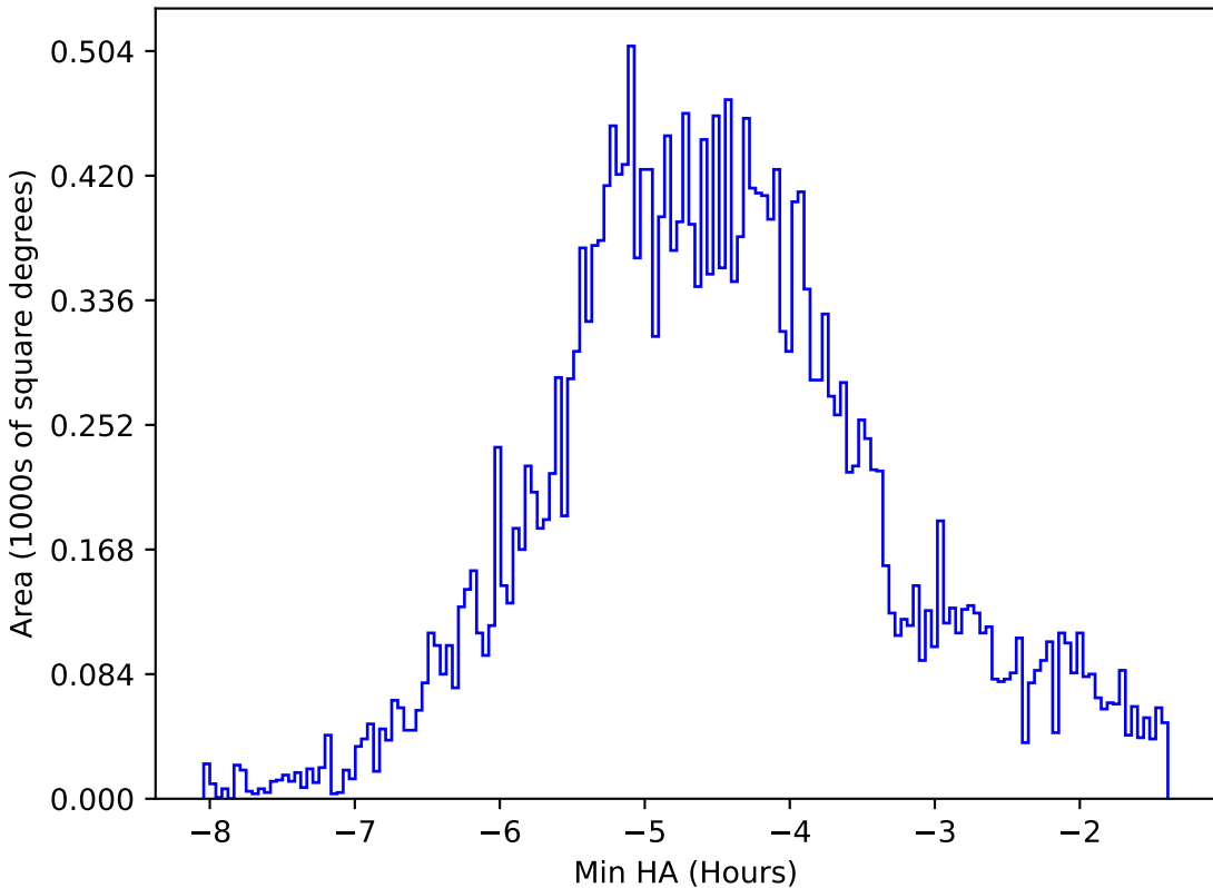
start_date_do90v3.4_10yrs All sky all bands: Min HA
