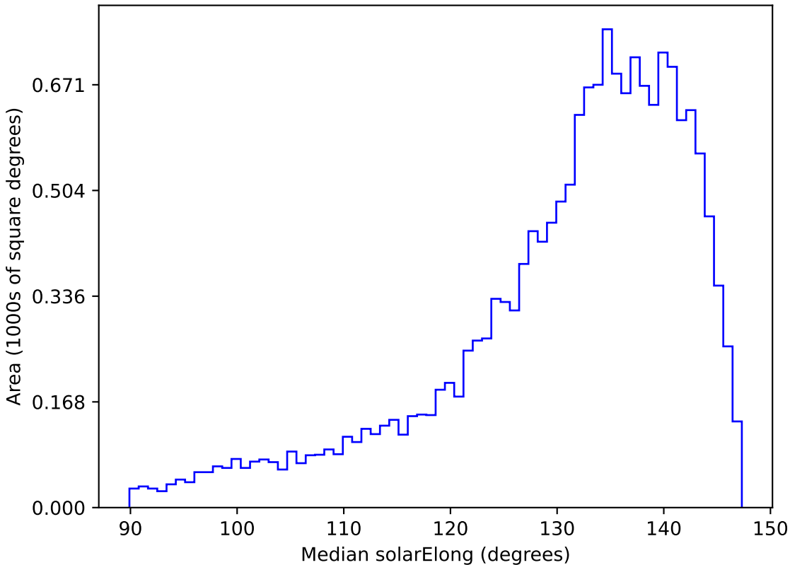
start_date_do90v3.4_10yrs WFD r band: Median solarElong
