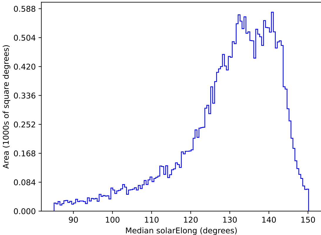
start_date_do90v3.4_10yrs All sky all bands: Median solarElong
