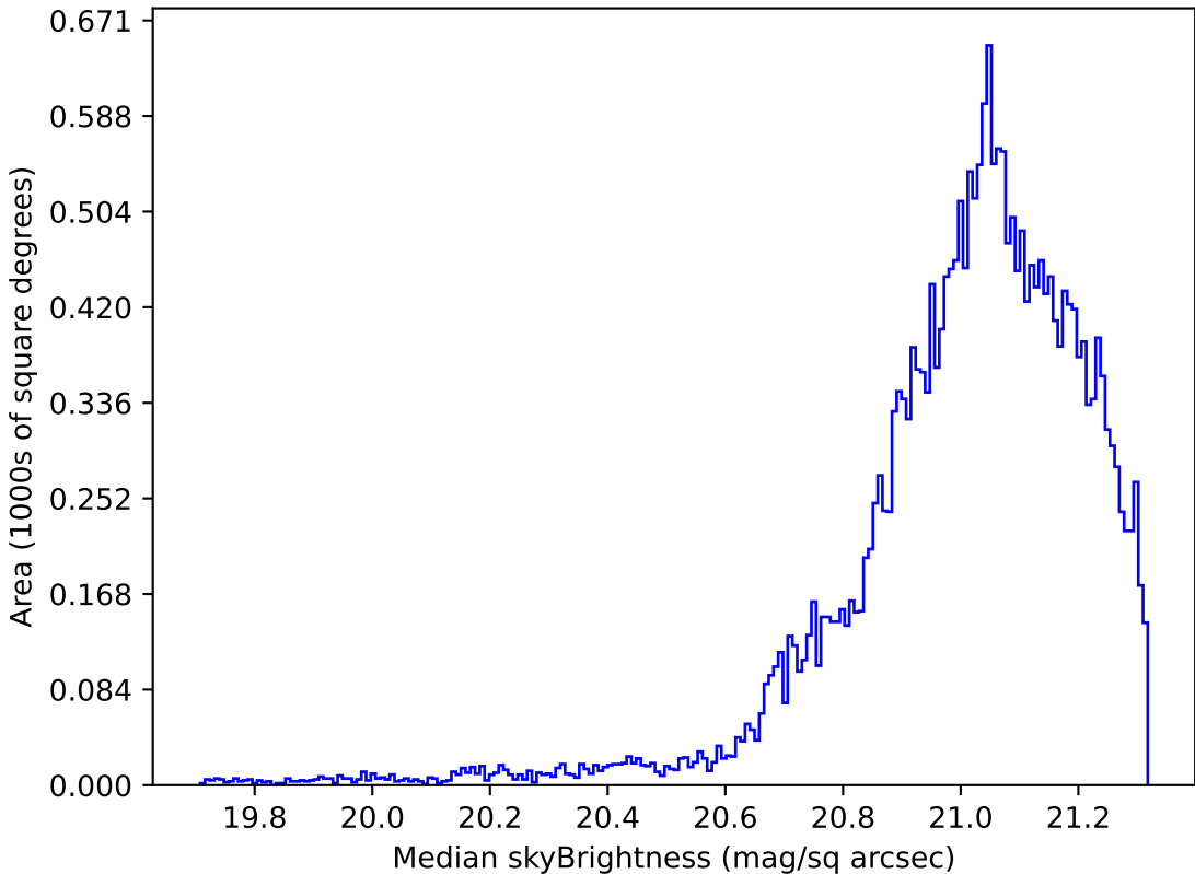
start_date_do90v3.4_10yrs Yr 1 r band: Median skyBrightness
