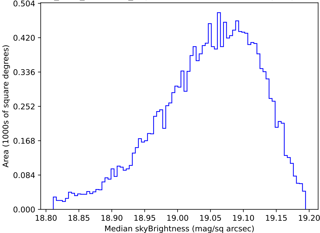
start_date_do90v3.4_10yrs WFD z band: Median skyBrightness
