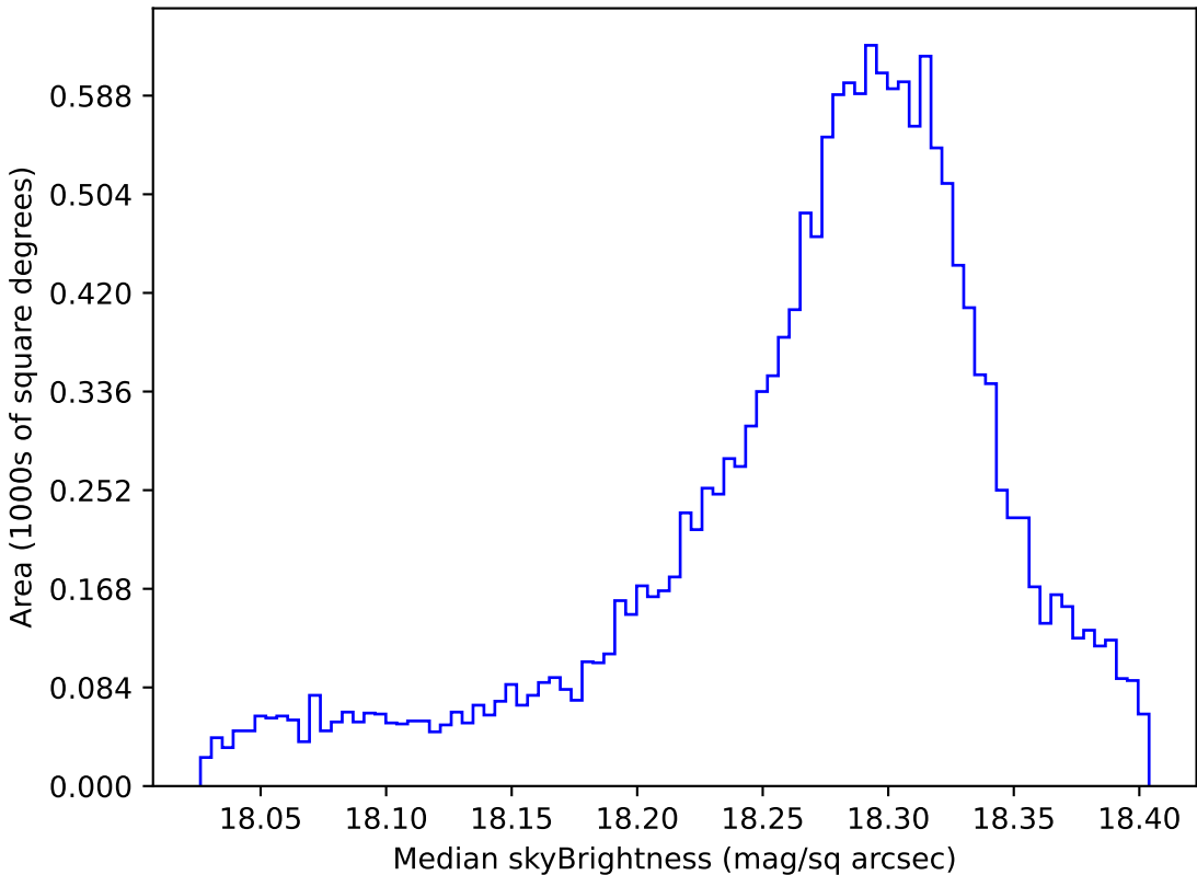
start_date_do90v3.4_10yrs WFD y band: Median skyBrightness
