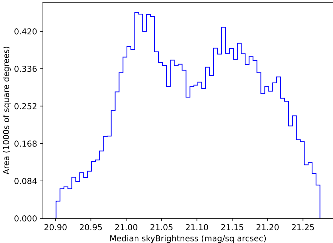
start_date_do90v3.4_10yrs WFD r band: Median skyBrightness
