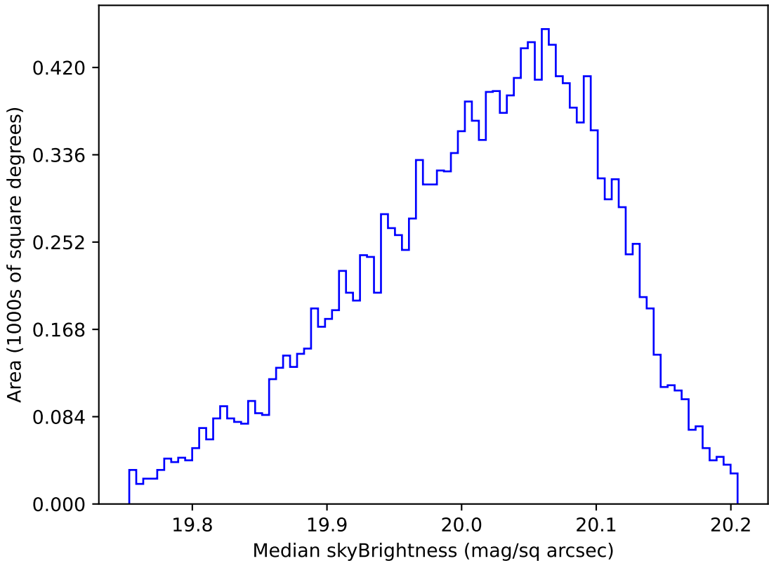
start_date_do90v3.4_10yrs WFD i band: Median skyBrightness
