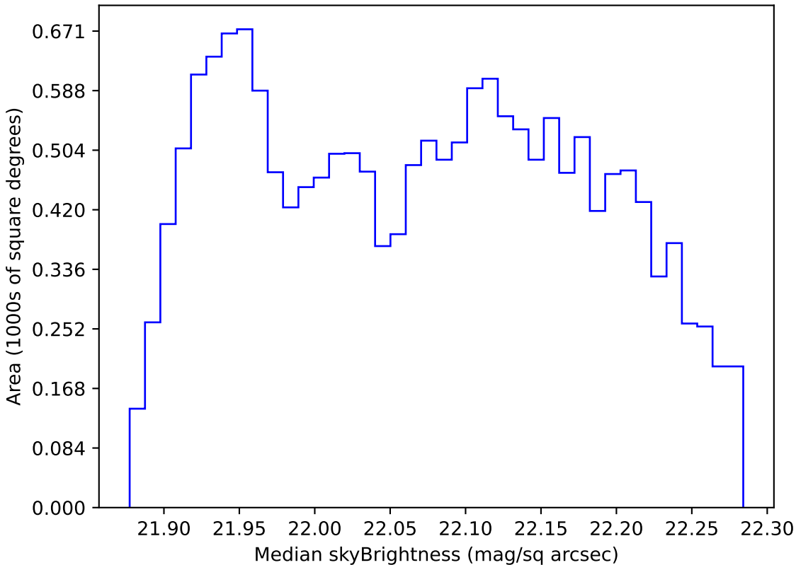
start_date_do90v3.4_10yrs WFD g band: Median skyBrightness
