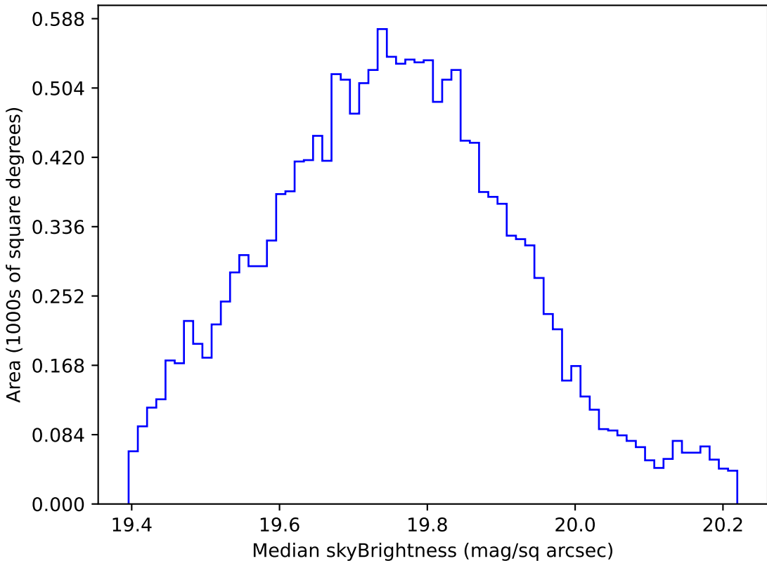
start_date_do90v3.4_10yrs WFD all bands: Median skyBrightness
