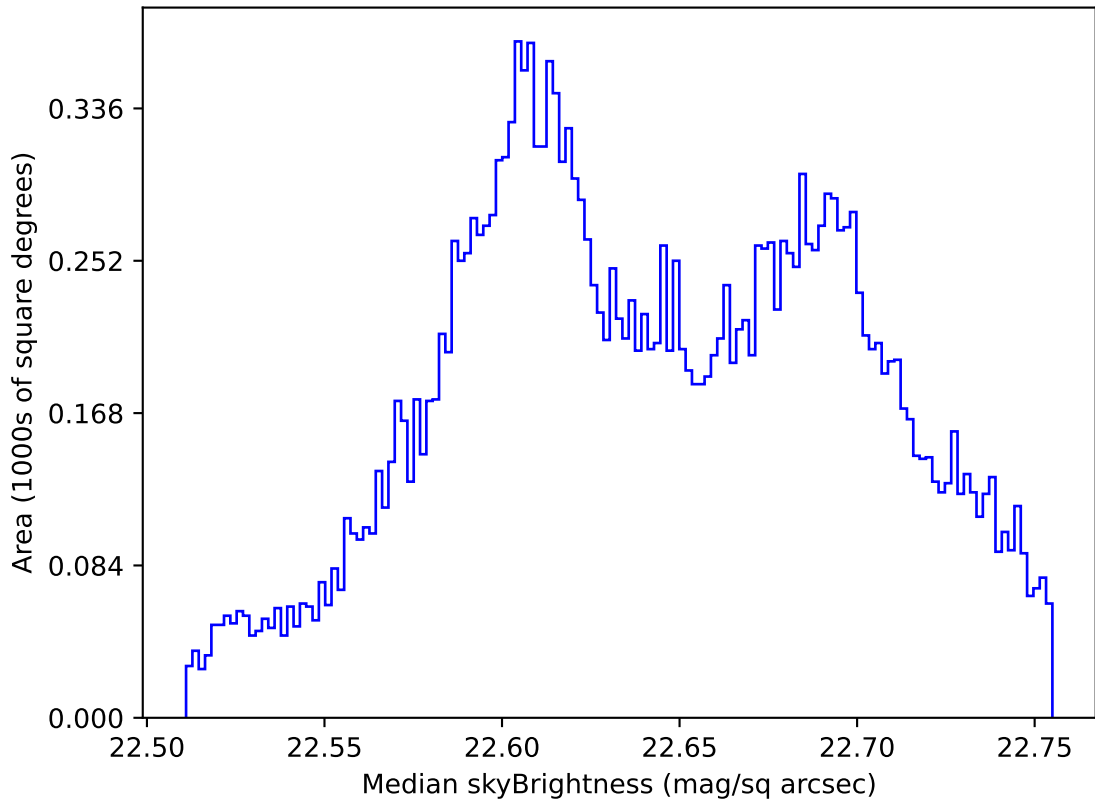
start_date_do90v3.4_10yrs All sky u band: Median skyBrightness
